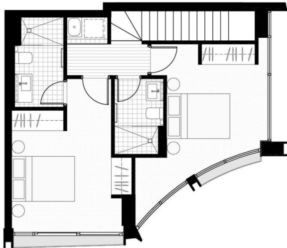
UPPER FLOOR
