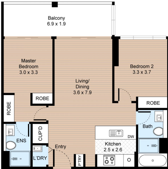
FLOOR PLAN
