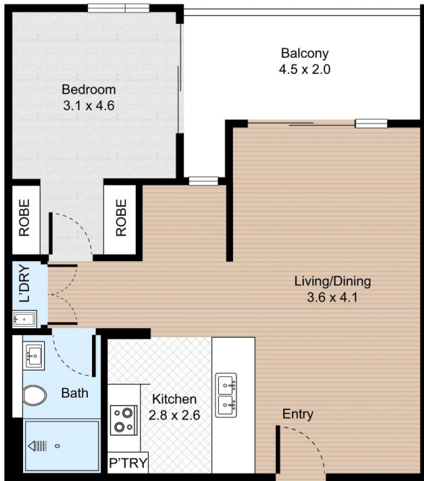
FLOOR PLAN
